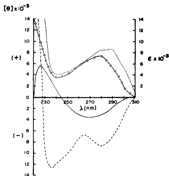
Figure 5. Uv and CD spectra of formycin B (8) and 2,5'-anhydroformycin B (9) in water. Spectra in 0.01 N HCl are identical with those in water: (—O—O—), 8 (uv); (·····), 9 (uv); (—), 8 (CD); (- - -), 9 (CD).
